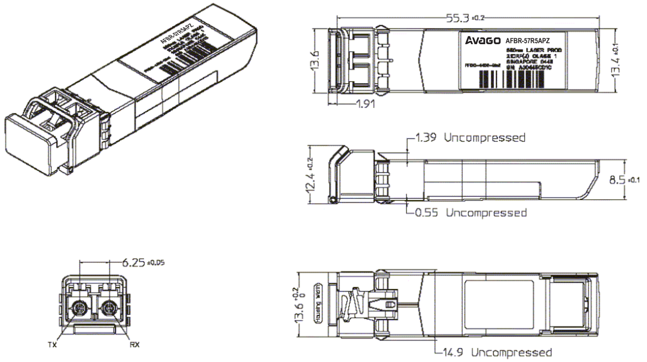
Figure 5. Module drawing.
